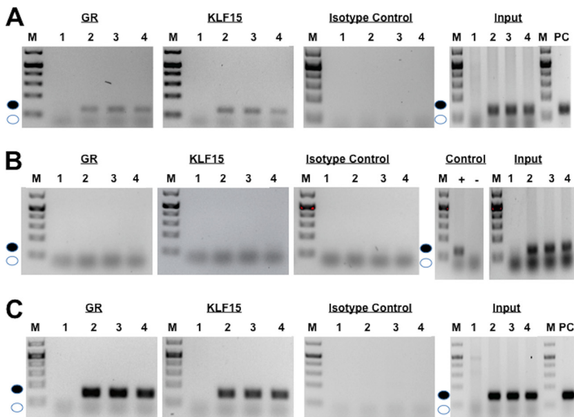
FIG 9 Interaction between GR and KLF15 with IETu1 GREs and UL52 sequences. Neuro-2A cells were cotransfected with the IETu1 GRE construct (A; 4 \mu g of DNA), the \Delta 2 \times \text{GRE} \Delta \text{KLF} (B; 4 \mu g of DNA), or the UL52 plasmid (C; 4 \mu g of DNA) and KLF15 and/or the GR plasmid (1 \mu g of DNA). Empty vector was added to maintain the same concentration of DNA in each transfection assay. Designated cultures were treated with DEX as described above. (A) Neuro-2A cells were transfected with no plasmid (lanes 1), with the IETu1 GRE construct (lanes 2), with IETu1 GREs, KLF15, and the GR (no DEX treatment) (lanes 3), and with IETu1 GREs, KLF15, and the GR (lanes 4). Cultures were treated with DEX (10 \mu M) in 2% stripped-serum medium for 4 h before cells were harvested. (B) Neuro-2A cells were transfected with no plasmid (lanes 1), with the \Delta 2 \times \text{GRE} \Delta \text{KLF} construct (lanes 2), with \Delta 2 \times \text{GRE} \Delta \text{KLF} , KLF15, and the GR (no DEX treatment) (lanes 3), and with \Delta 2 \times \text{GRE} \Delta \text{KLF} , KLF15, and the GR (lanes 4). Cultures were treated with DEX (10 \mu M) in 2% stripped-serum medium for 4 h before cells were harvested. (C) Neuro-2A cells were transfected with no plasmid (lanes 1), with a UL52 construct (lanes 2), with UL52, KLF15, and the GR (no DEX treatment) (lanes 3), and with UL52, KLF15, and the GR (lanes 4). Cultures were treated with DEX (10 \mu M) in 2% stripped-serum medium for 4 h before cells were harvested. Transfected cells were processed for ChIP as described in the Materials and Methods section, and immunoprecipitation (IP) was conducted using the GR antibody, KLF15 antibody, or isotype control antibody. Input was 10% of the total DNA-protein complexes that were used for IP, and then PCR was performed using PCR primers described in the Materials and Methods section. The filled circle denotes the specific PCR fragment of 107 bp for the IETu1 GREs, 107 bp for \Delta 2 \times \text{GRE} \Delta \text{KLF} , or 132 bp for UL52, and the open circle denotes the position of primer dimers. These results are representative of five independent studies for the GR ChIP and of two for the KLF15 ChIP and \Delta 2 \times \text{GRE} \Delta \text{KLF} . M, molecular mass marker.
